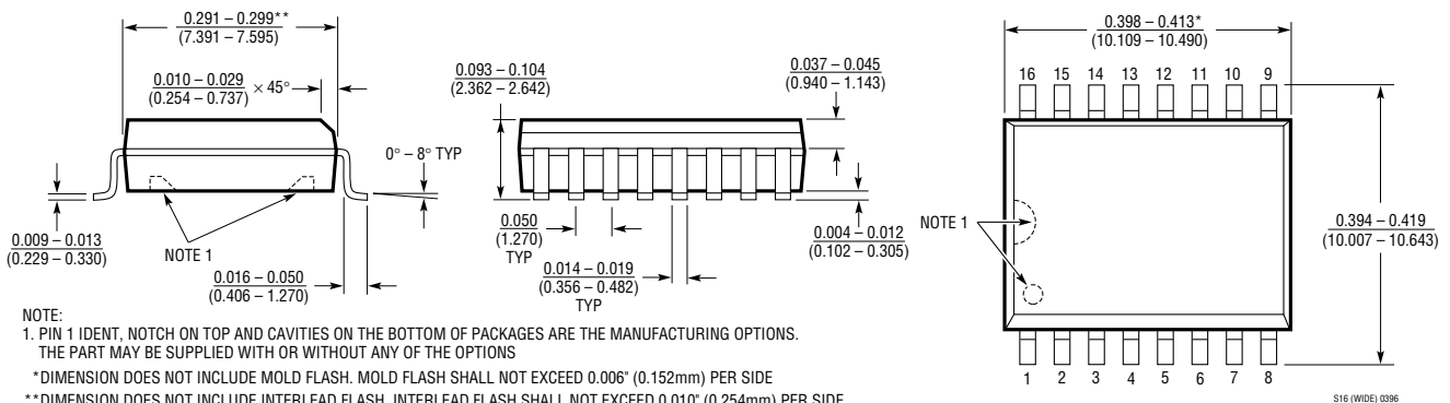
SW Package 16-Lead Plastic Small Outline (Wide 0.300) (LTC DWG # 05-08-1620)
