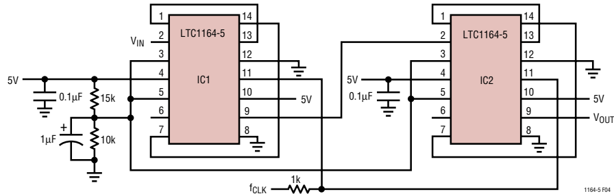
Single 5V, I_S = 5.2\text{mA} , 16th Order Clock-Tunable Lowpass Filter, f_{\text{CLK}}/f_{\text{CUTOFF}} = 60:1 , -75\text{dB} Attenuation at 2.3 f_{\text{CUTOFF}}
